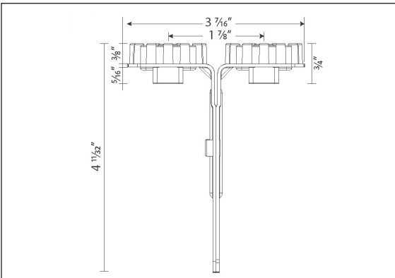
A72R DIMENSIONS
