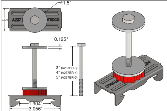
A237BR DIMENSIONS
