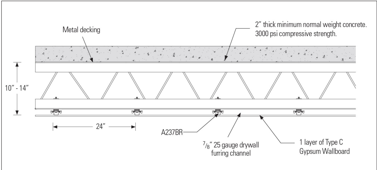
A237BR INSTALLATION DETAIL
