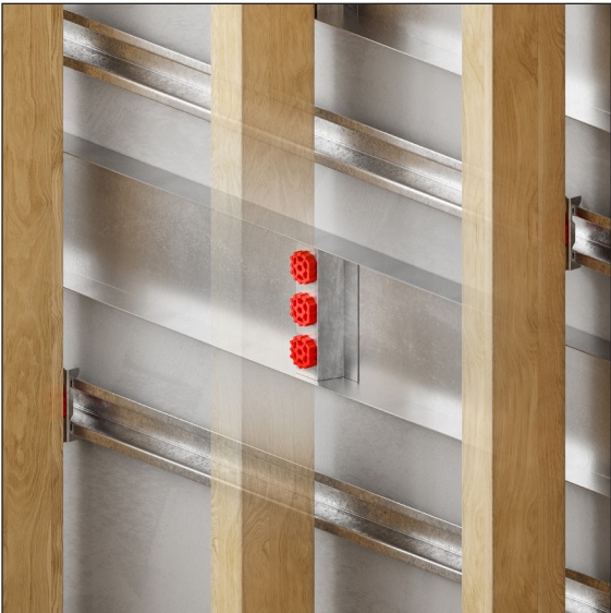
A106R INSTALLATION
