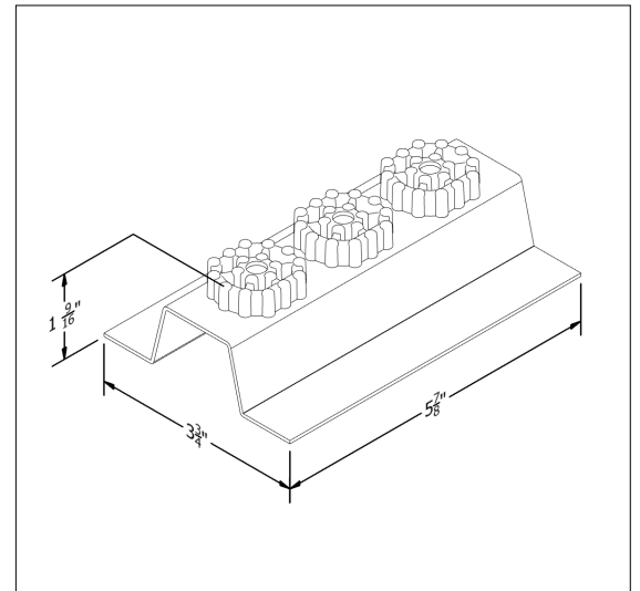
A130R DIMENSIONS
